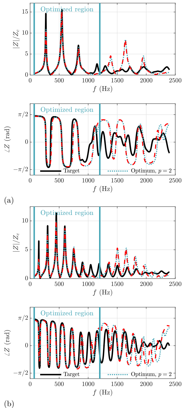
Figure 11: Comparison between target impedance (solid line), impedance for the optimized bicylindrical resonator without tone holes (blue dotted line) and with toneholes (red dashed line), for (a) the A fingering and (b) the low B fingering.
