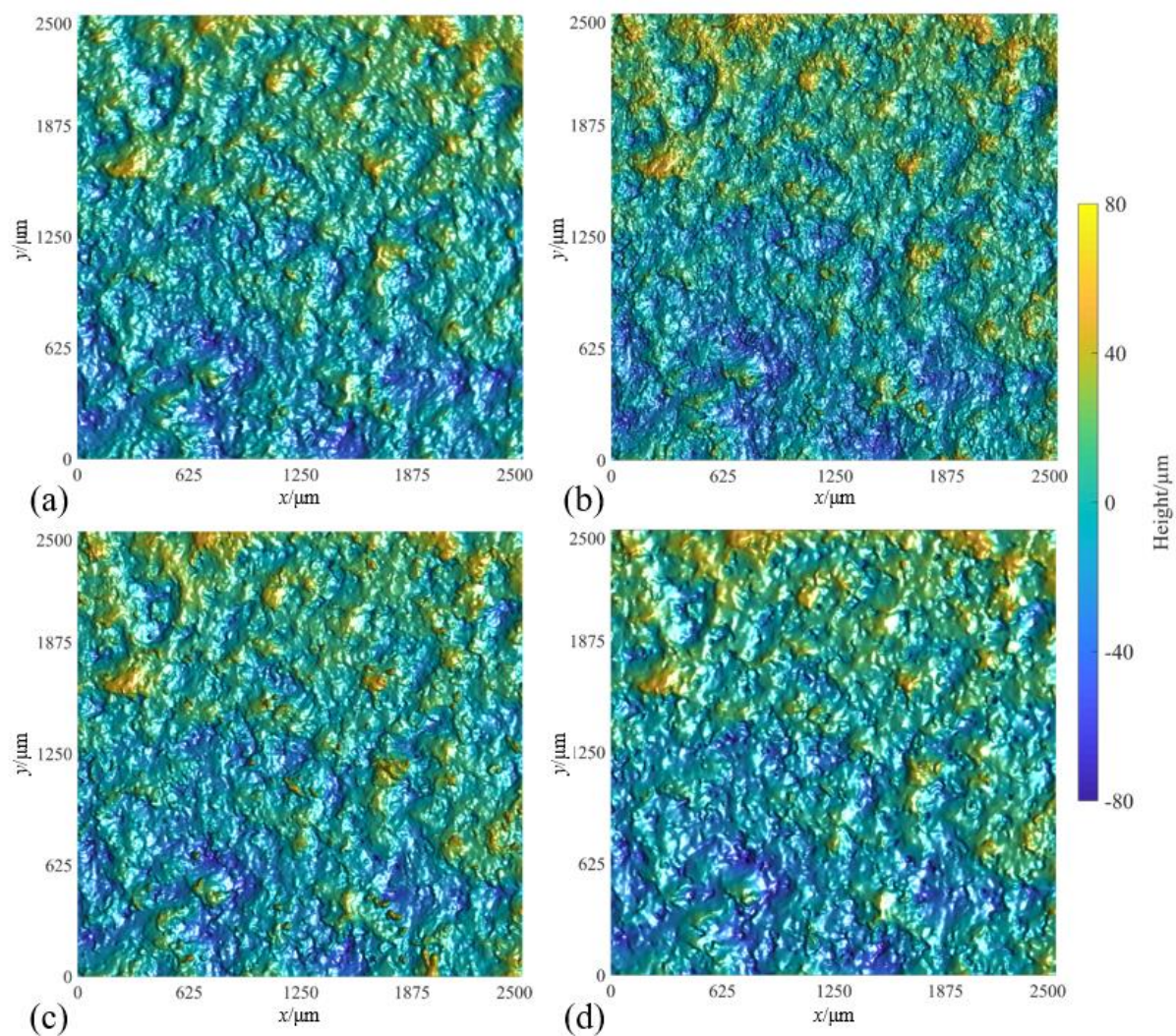
Figure 5: Example unfiltered top surface topographies: (a) CM, (b) CSI, (c) FV and (d) XCT.
