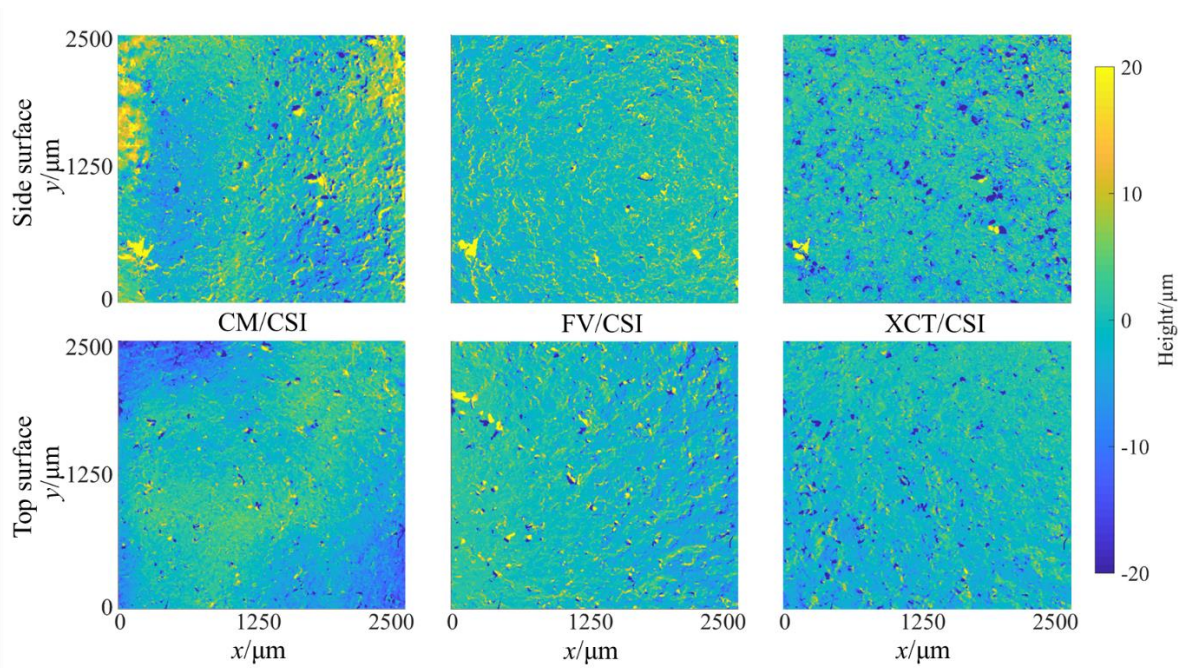
Figure 13: Local bias between spatial frequency band matched instrument pairs, comparing each measurement to CSI.
