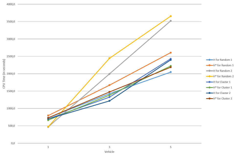
Figure 4.: Average CPU Times (in seconds) for All \mathcal{K}
