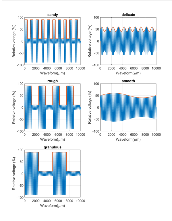
Figure 5: Waveform sample resulting from the parameters which can be used to elicit perceptions represented by the adjectives in Table 4
