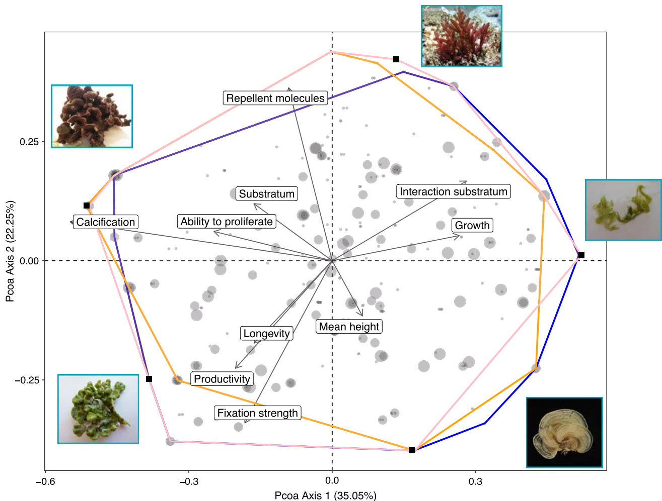
Fig. 5 Functional space and distribution of species inside the functional space of Europa, Glorioso and Juan de Nova (orange, blue, and pink, respectively). Circles represent species and are proportional to their respective occurrence at the three reefs. Large circle = species has been collected at the three reefs, medium circle: species has been collected at two reefs, and small circle: species has been collected at
