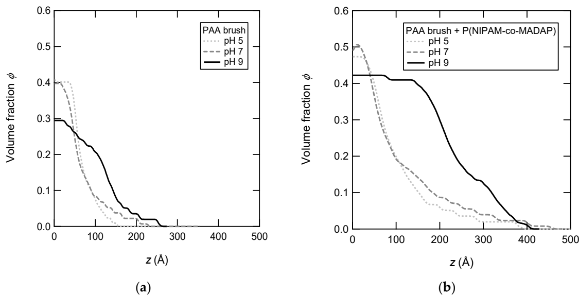
Figure 9. (a) Density profiles of a PAA brush ( N = 328 , \gamma = 37 \text{ Å} , \sigma = 0.125 \text{ nm}^{-2} ) without adsorbed copolymers and (b) with adsorbed copolymers at various pH: pH 5 (dotted line), 7 (dashed line), and 9 (full line).
