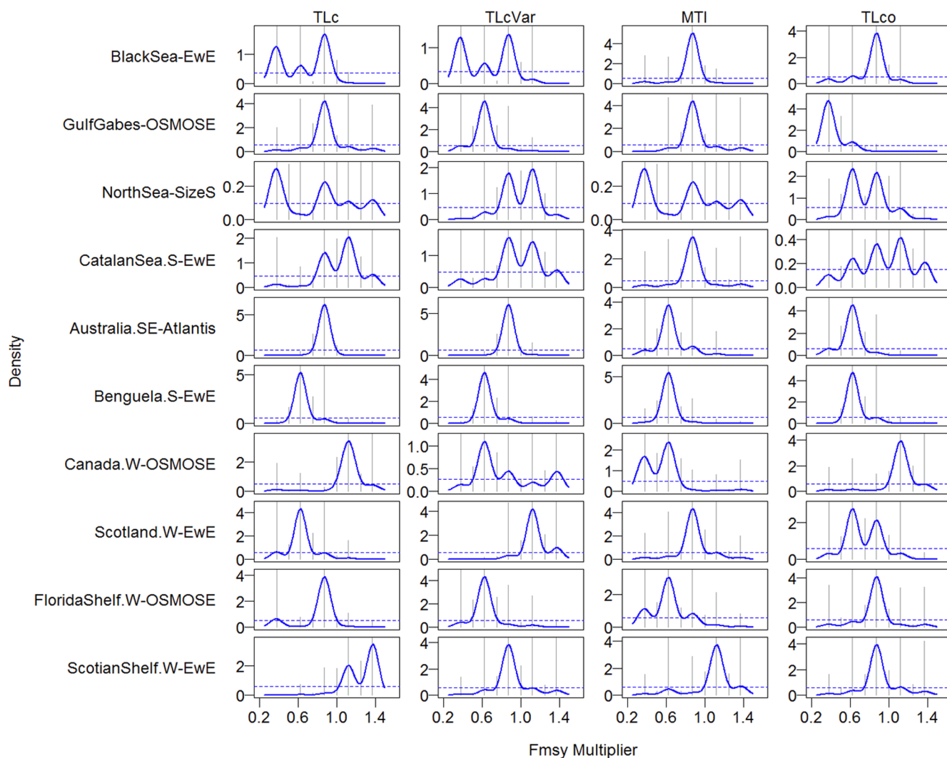
Fig. 6. Threshold shifts in the values of four trophic level (TL) based indicators (TLC: mean TL of catch, TLcVar: mean TL of catch with variable TL, MTI: marine trophic index, and TLco: mean TL of fish community surveyed) along the gradient of fishing pressure under directional change in primary productivity. The dashed line indicates where the ratio of the density of split importance to the density of observed fishing pressure is 1; peaks above the dashed line suggest threshold values for the fishing pressure.
