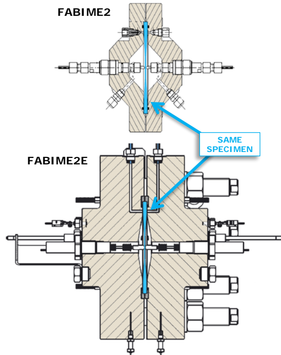
Figure 10: Comparison between FABIME2 and FABIME2E fatigue cells (same scale and specimen geometry)
