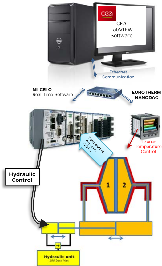
Figure 12: Software overview
