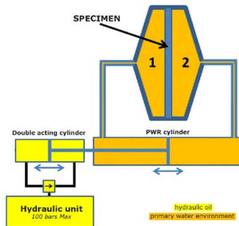
Figure 8: Double cylinder system for separation of PWR and Hydraulic fluid
