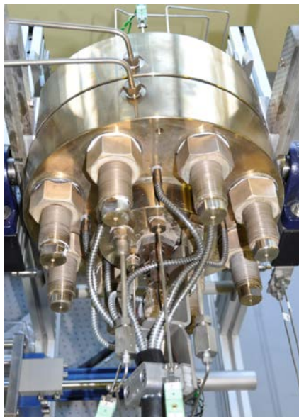
Figure 11: Detail of the FABIME2E cell - attachment stud
