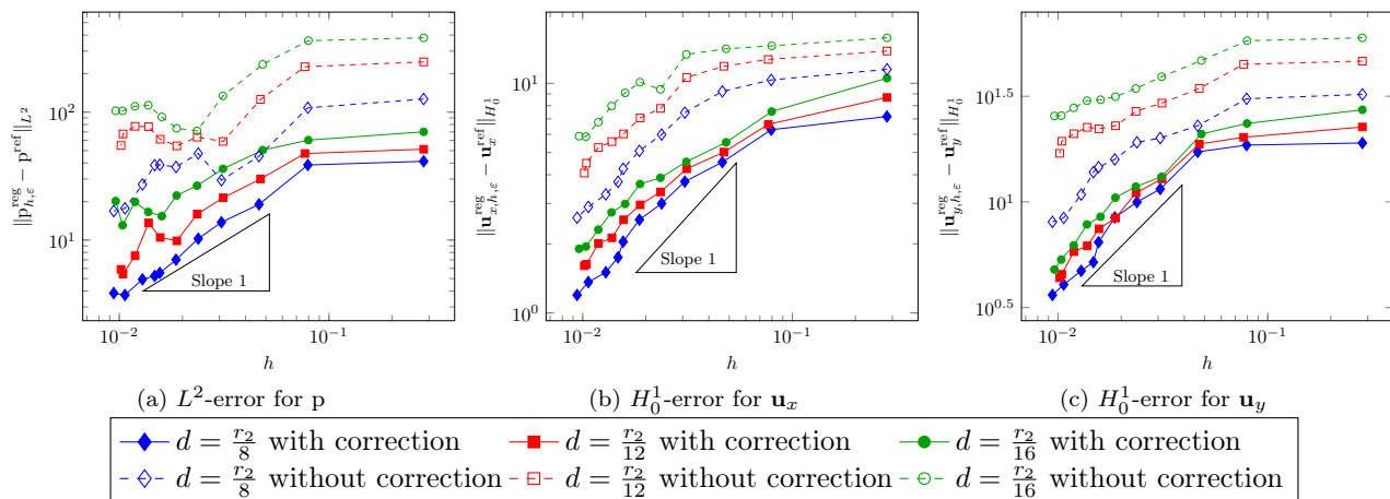
Figure 14: Absolute error in function of h for 3 different distances for 3 aligned particles
