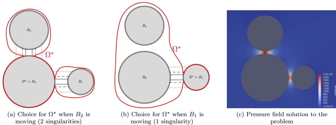
Figure 16: Three particles in an L-shape configuration.
