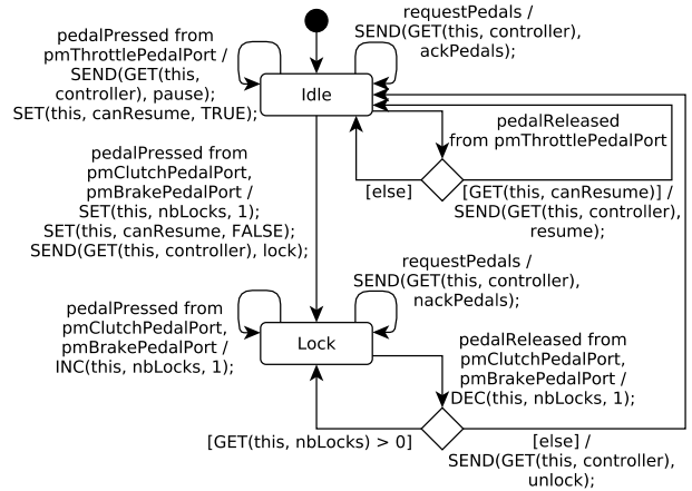
(a) State machine of the PedalsManager class.
