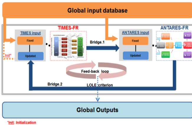
Figure 1 Schematic overview of TIMES-ANTARES linking model. The uninterrupted line describes the information flow interactions, the dashed line indicates the initialization step which is considered as the beginning of the linking process. The first step of the iteration is a TIMES solution. ANTARES is then run with a TIMES solution for a target year, and operates a Monte Carlo dispatch. The iteration ends as soon as the LOLE criterion is achieved. The global outputs are the power generation mix obtained and the insights offers by the linking model.
