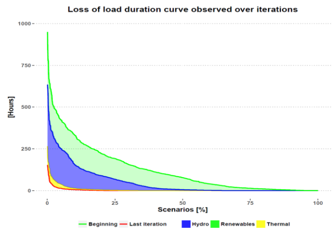
Figure 3 Loss of load duration curve evolution over iterations
