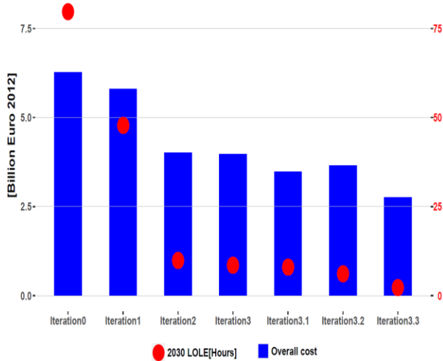
Figure 3 ANTARES overall operational costs (2030) over iterations.
