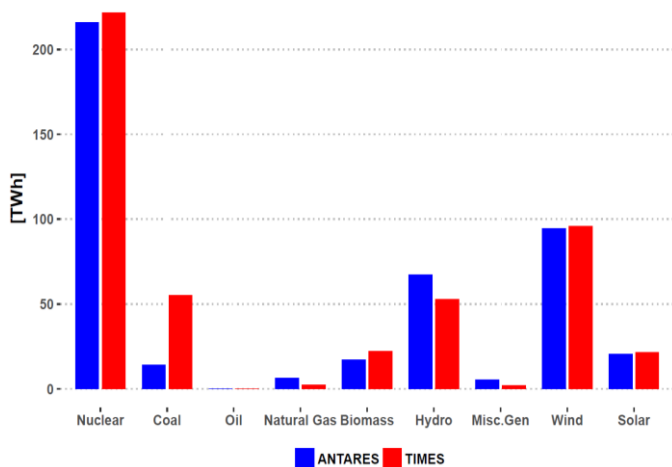
Figure 2 Annual power generation comparison between TIMES (red) and ANTARES median scenario (blue)
