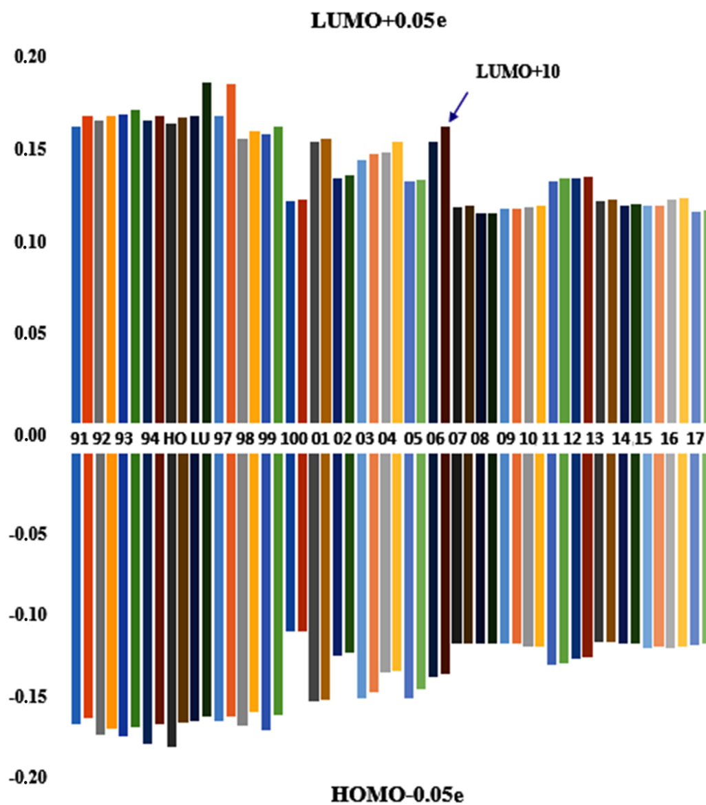
Fig. 8 Relaxation of the (\alpha, \beta) orbitals of the B complex (Cyclohexyl link) when frontier orbitals are altered by 0.05 electron occupancy. (Eigen value shifts in eV).
