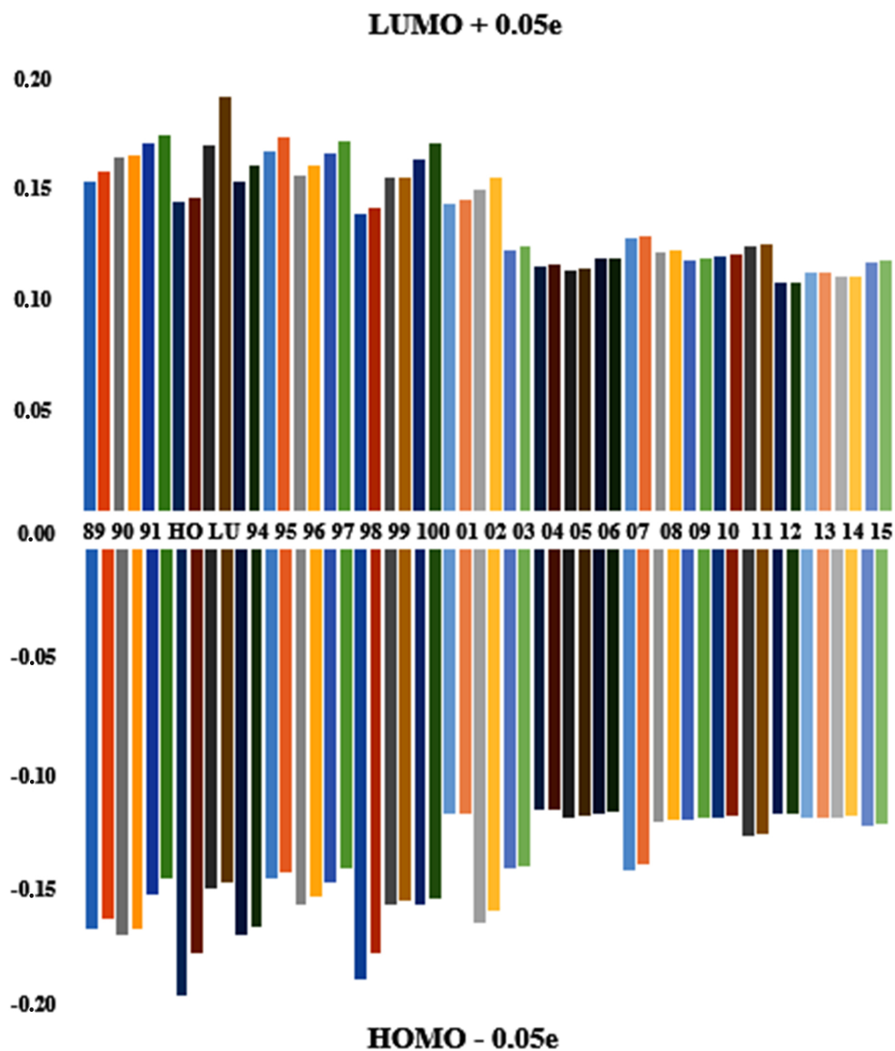
Fig. 9 Relaxation of the (\alpha, \beta) orbitals of the D complex (pyridyl link) when frontier orbitals are altered by 0.05 electron occupancy. (Eigen value shifts in eV).
