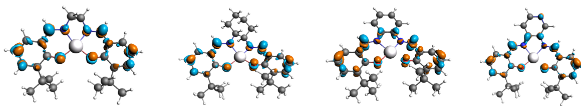
Fig. 2a DD of Zn selected sal(ph) complexes calculated according eq. (5); isovalue 3 \cdot 10^{-3} a.u.
