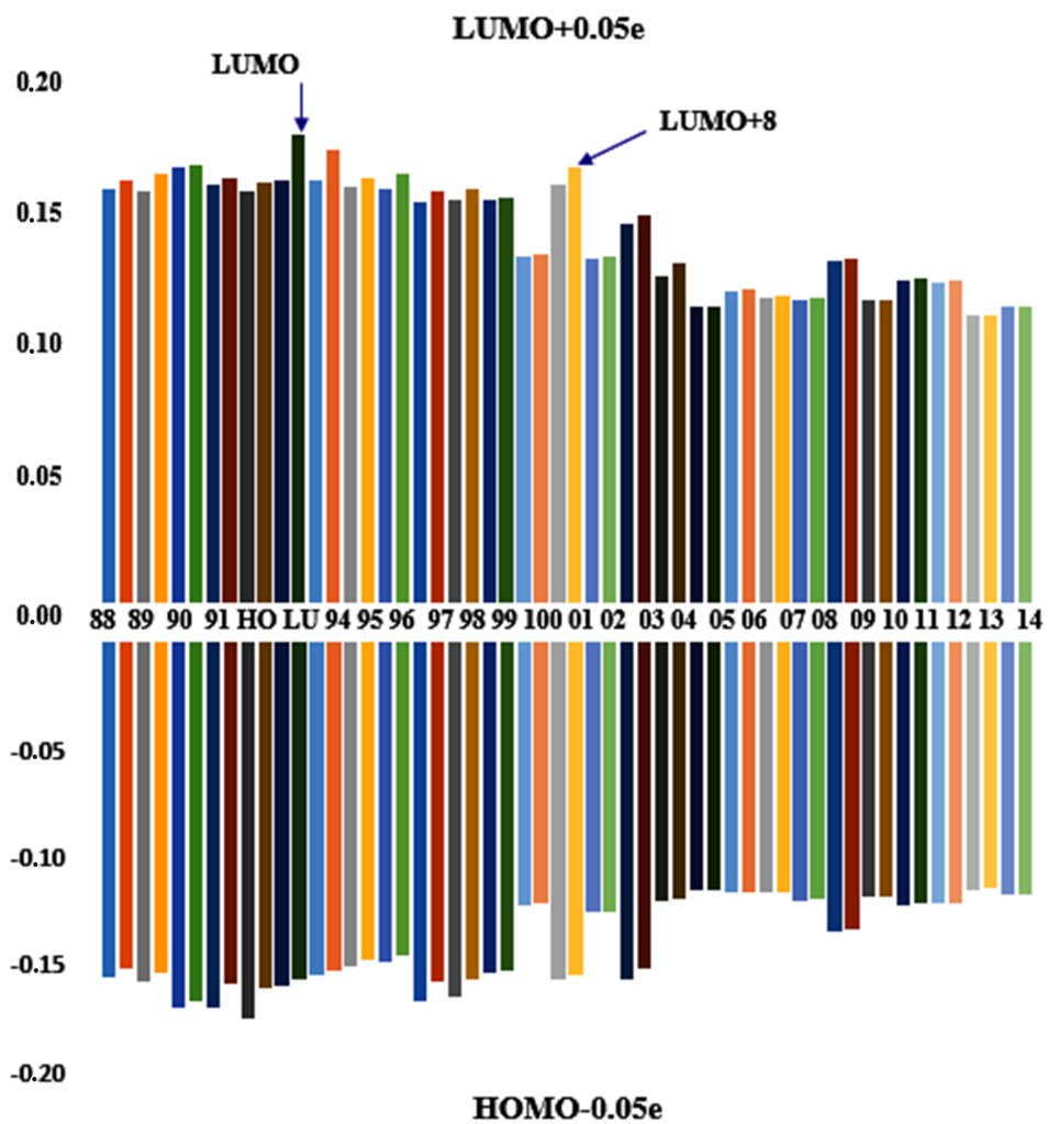
Fig. 7 Relaxation of the (\alpha, \beta) orbitals of the C complex (Phenyl link) when frontier orbitals are altered by 0.05 electron occupancy. (Eigen value shifts in eV).
