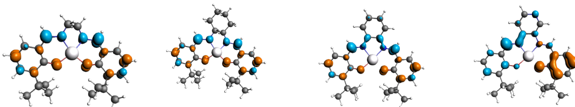
Fig. 2b DD of Zn selected sal(ph) complexes calculated according eq. (6); isovalue 3 \cdot 10^{-3} a.u.
