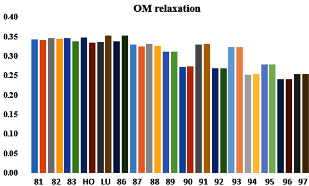
Fig. 6 MO relaxation through the 0.05e- HOMO (#84) → LUMO (#85) excitation of complex A (ethyl bridge)
