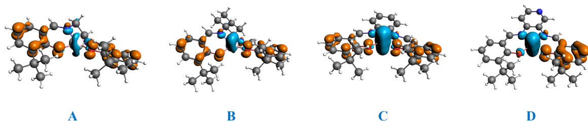
Fig. 4 SSDD for the n^{\text{th}} excited state of the investigated Zn- Sal(ph)en complexes with various diamine bridge (Ethyl(A), Cyclohexyl(B), Phenyl(C), Pyridyl(D)) (isovalue = 3.10^{-3}a.u. )
