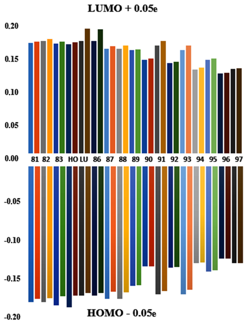
Fig. 5 Relaxation of the (\alpha, \beta) orbitals of the A complex when frontier orbitals are altered by 0.05 electron occupancy. (Eigen value shifts in eV).
