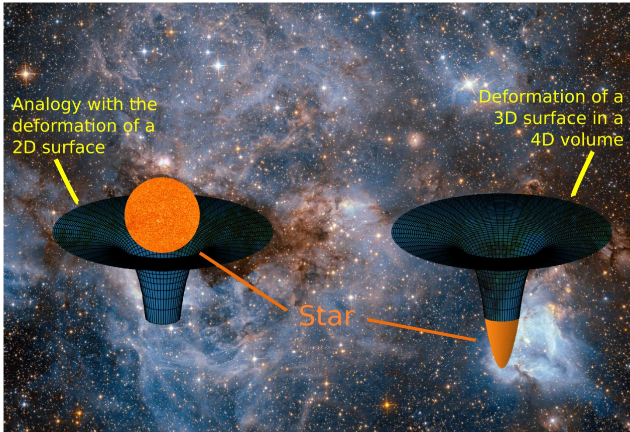
Fig. 1 Schematic representations of space deformation. Left: With a two-dimensional analogy for space but not for the star (general relativity). Right: With the analogy for both (more consistent).
