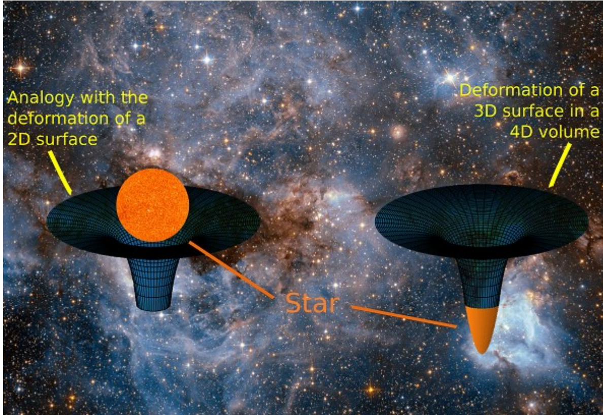
Fig. 1. Schematic representations of the space deformation. Left: With a two-dimensional analogy for space but not for the star (general relativity). Right: With the analogy for both (more consistent).
