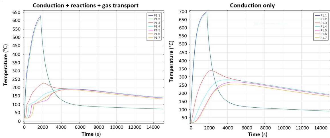
Figure 6 – Temperature evolution at several locations of the cask wall calculated with the full model and the conduction-only model - Polyester resin compound as shielding material
