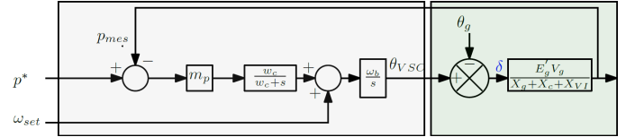
Fig. 5. Quasi-static model of the VSC based droop control
