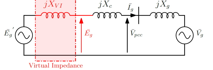
Fig. 4. Simplified quasi-static grid-forming model including VI
