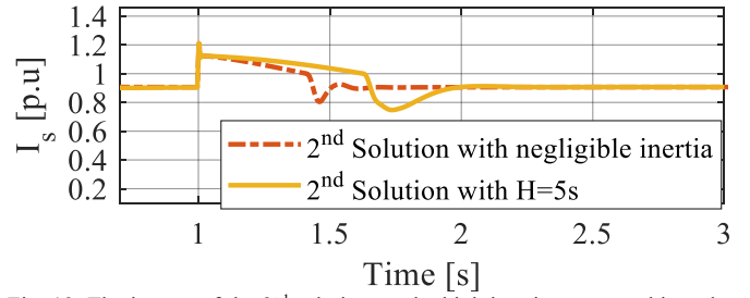
Fig. 19. The impact of the 2 nd solution on the high inertia system subjected to a 30^\circ phase shift.
