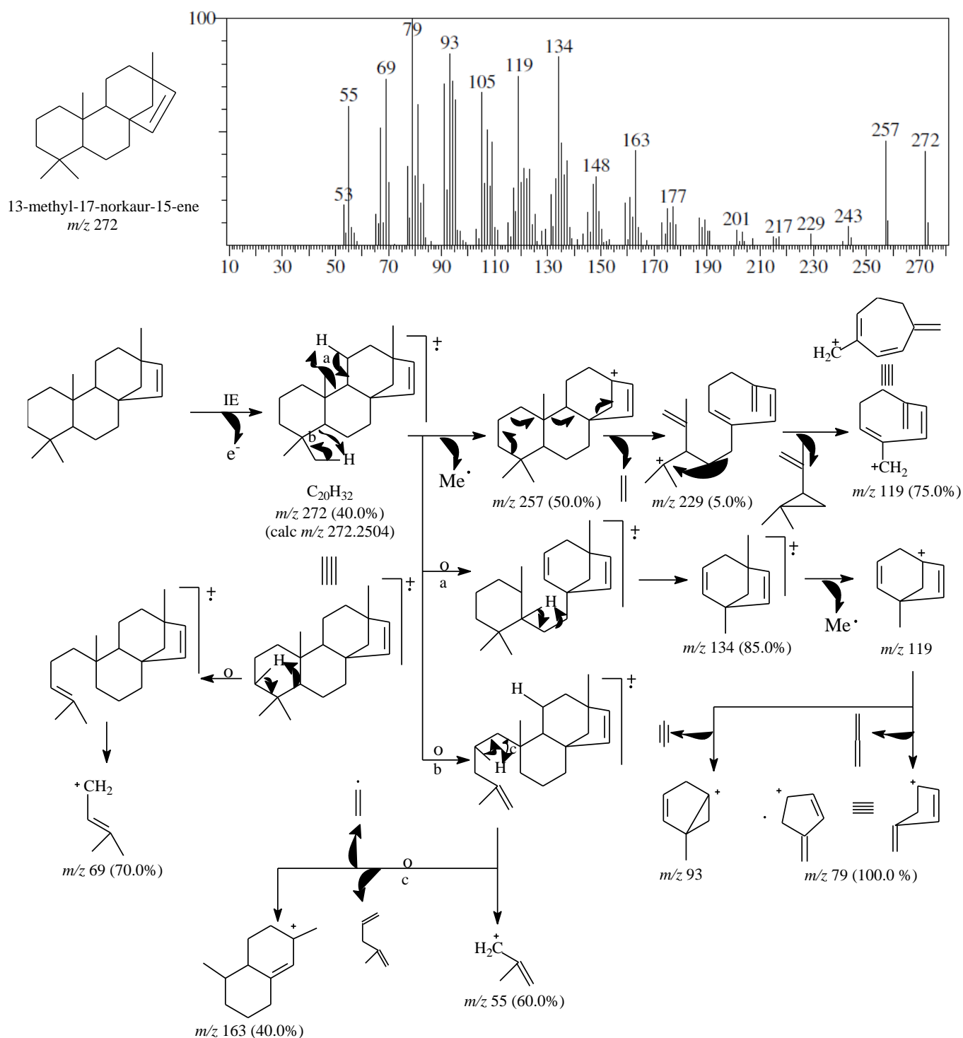
Figure 11. Mass spectra and fragmentation proposed for 13-methyl-17-norkaur-15-ene, identified in Hex-Sb.
