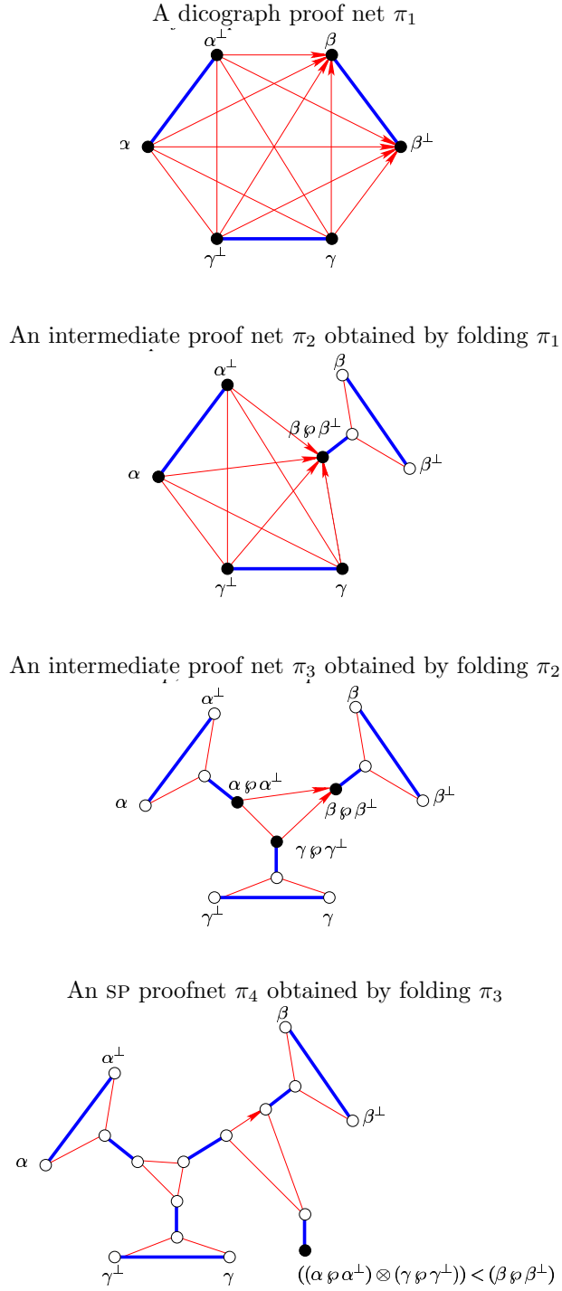
Figure 7: Progressively turning a dicograph proof net \pi_1 into a pomset proof net \pi_4 with one conclusion via some intermediate proof nets \pi_2 and \pi_3 . The conclusions of the pomset proof net and of the intermediate proof nets are emphasised by filled black dots.
