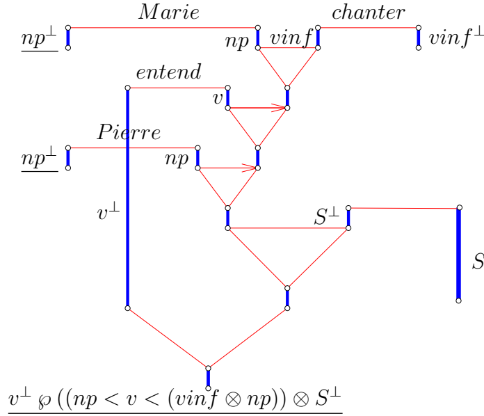
Figure 9: Analysis of a relatively free word order sentence — order Pierre < entend < (Marie \otimes chanter)
