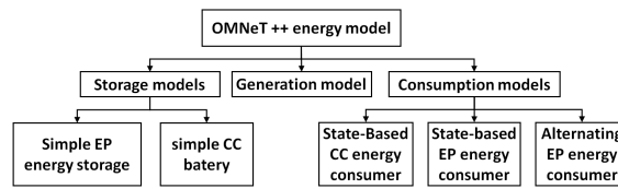
Figure 5: The hierarchical structure of OMNeT++ energy model
