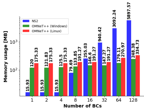
Figure 10: Memory usage of NS2 and OMNeT++
