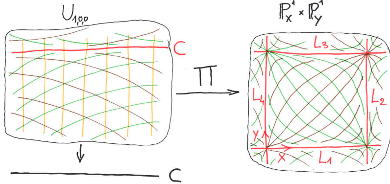
FIGURE 1. Serre isomorphism
