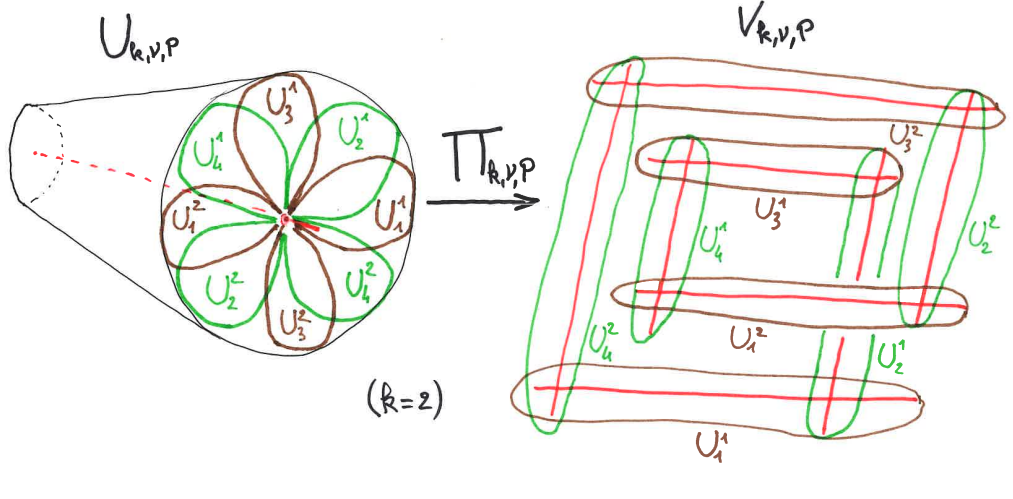
FIGURE 7. The isomorphism \Pi_{k,\nu,P} for k = 2
