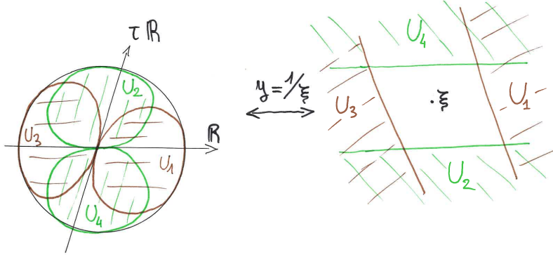
FIGURE 2. Neighborhoods correspondence
