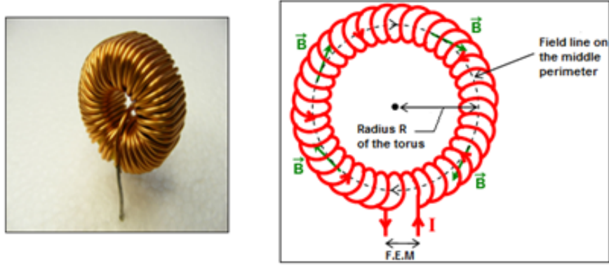
Fig. 1. A torical coil.
