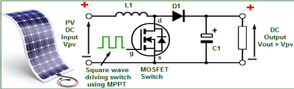
Fig. 3. Equivalent electrical circuit of boost converter.
