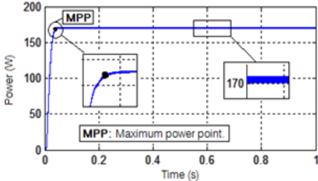
Fig. 11. The output power P_s of boost converter.
