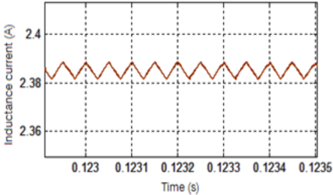
Fig. 14. Current through the inductor i_L .
