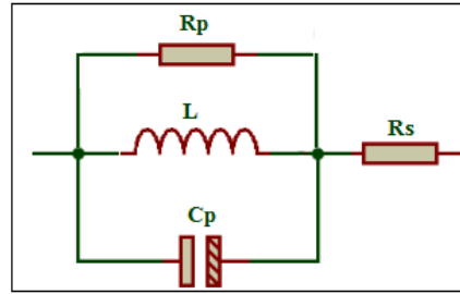
Fig. 7. Equivalent model of impedance Z .
