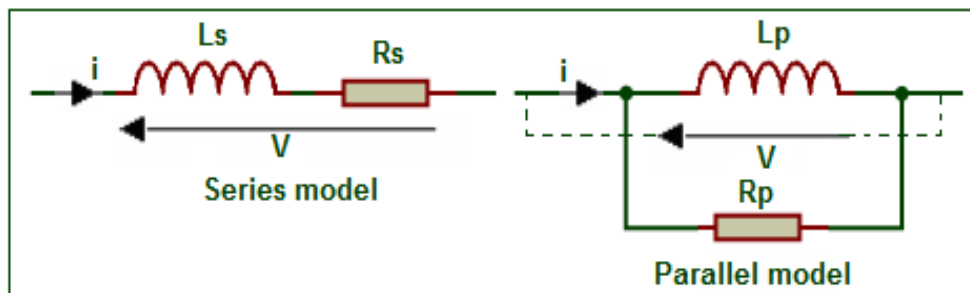
Fig. 2. Dipole models (series, parallel).
