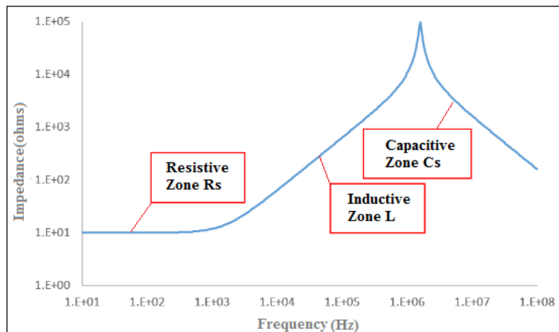
Fig. 8. The module of the impedance Z .
