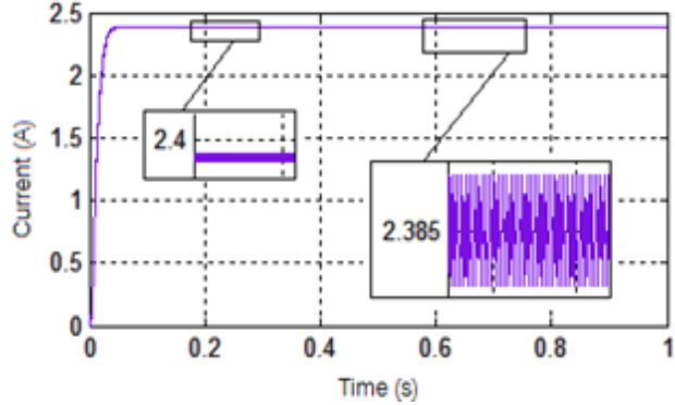
Fig. 13. The output current I_s of boost converter.
