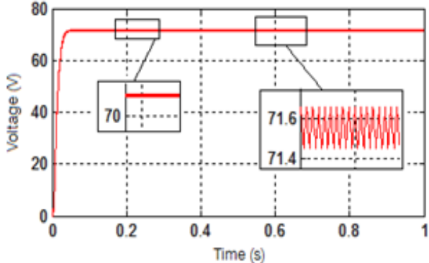
Fig. 12. The output voltage V_s of boost converter.
