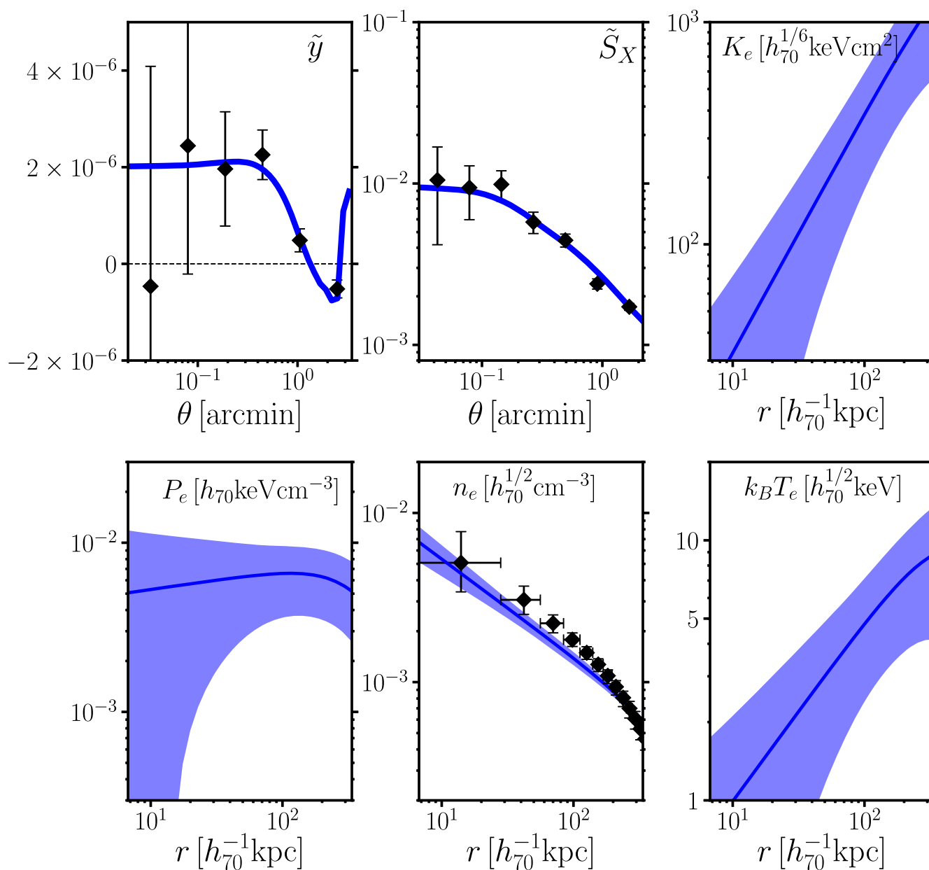
Figure 14. The same figure as Fig. 3, but for HSC J021056-061154. The signal-to-noise ratios of the y and S_X profiles are \sim 5\sigma and \sim 16\sigma , respectively. The increase in the \tilde{y}_m profile at large radii is caused by the transfer function.
