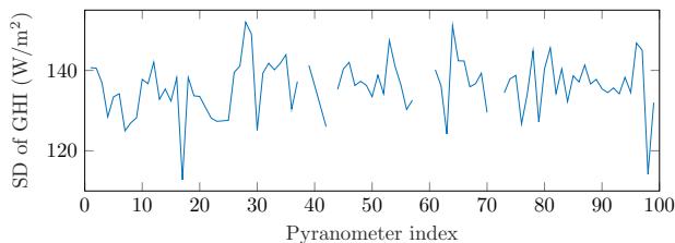
FIG. 8. Standard deviation (SD) of the satellite estimations error over time as a function of the location. Missing points refer to pyranometers that were excluded.
