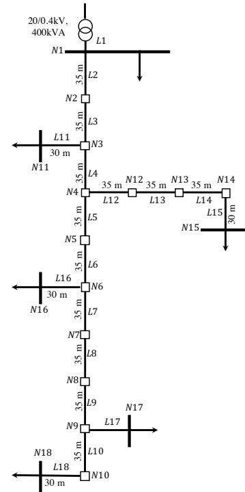
FIG. 5. The CIGRE benchmark grids for LV systems 11 .
