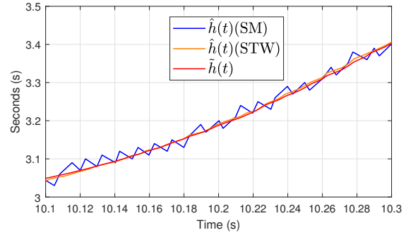
(c) Chattering analysis for fast-varying delay estimation on interval t \in [10.1, 10.3] .
