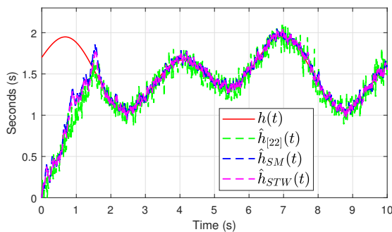
(a) Delay estimation via the three methods (delay measurement approach: \hat{h}_{[22]}(t) , standard sliding mode: \hat{h}_{SM}(t) and super-twisting method: \hat{h}_{STW}(t) ) in the presence of channel inherent noises.
