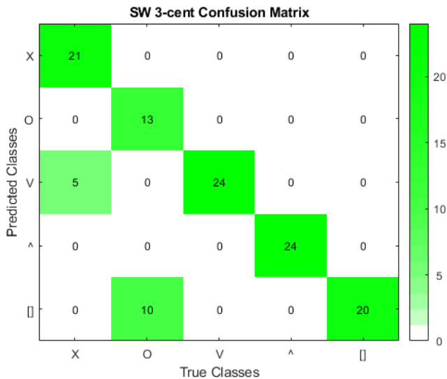
Figure 9: Confusion matrix of the Sliding Window 3-cent run, considering only the classification attempts in the correct time window.
