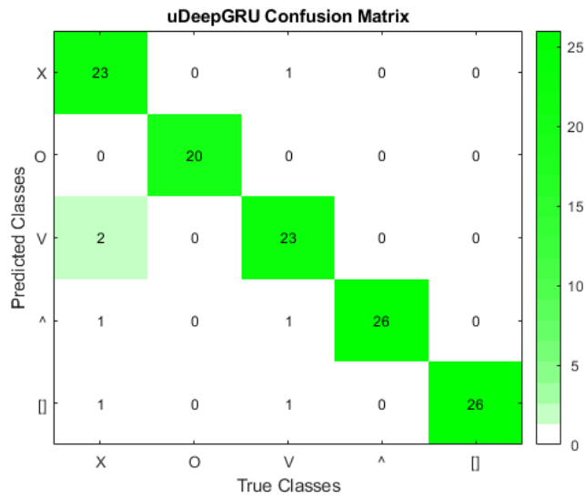
Figure 5: Confusion matrix of the uDeepGRU 2 run, considering only the classification attempts in the correct time window.
