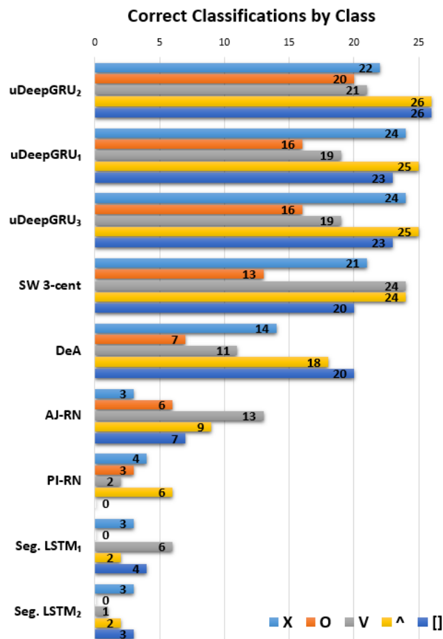
Figure 4: Number of correct detection and labellings by class for each method. It is possible to see that the recognition of the different gestures is not constant. Circle gestures are more likely not correctly detected, while caret and square are the ones more easily recognized by uDeepGRU and DeA. V-gestures are quite accurately detected by SW-3cent.
