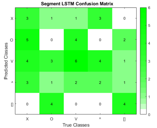
Figure 8: Confusion matrix of the Segment LSTM 1 run, considering only the classification attempts in the correct time window.
