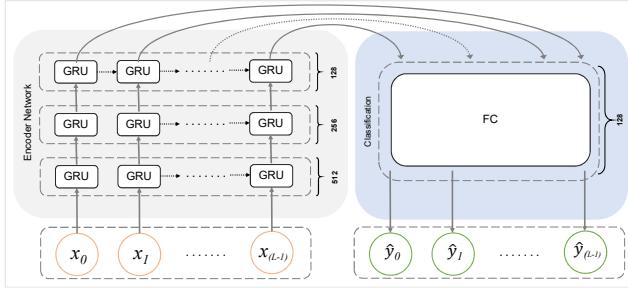
Figure 3: uDeepGRU architecture which consists of an encoder network and a classification subnetwork.
