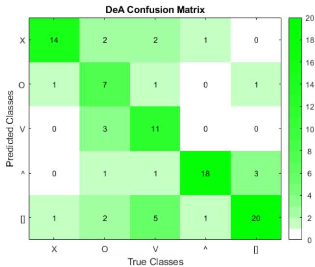
Figure 6: Confusion matrix of the DeA run, considering only the classification attempts in the correct time window.
