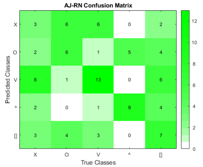
Figure 7: Confusion matrix of the AJ-RN run, considering only the classification attempts in the correct time window.
