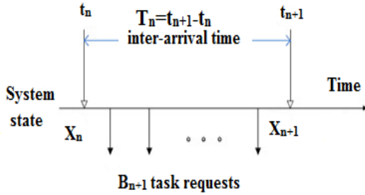
Figure 1: Embedded Markov points.
