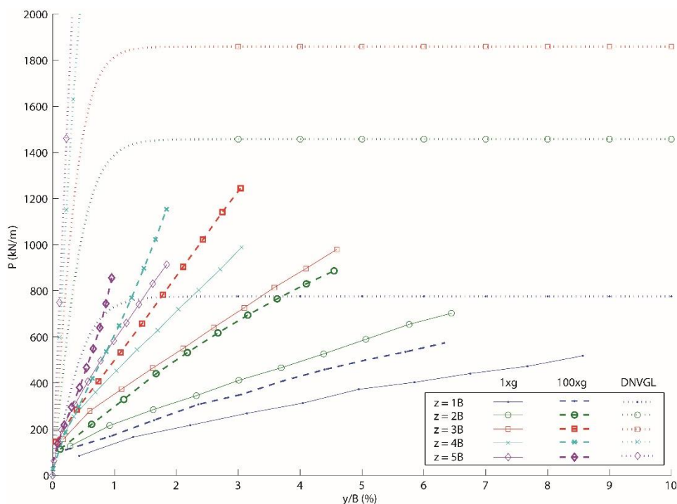
Figure 5. P-y curves
