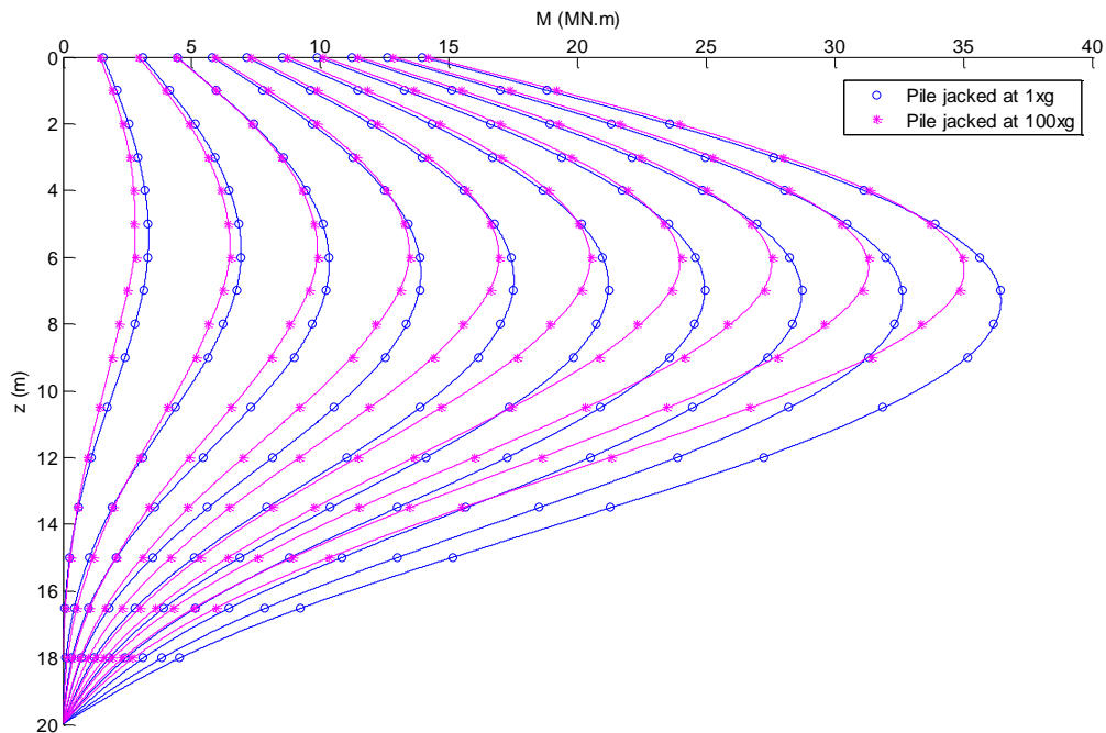
Figure 3. Moment profiles
