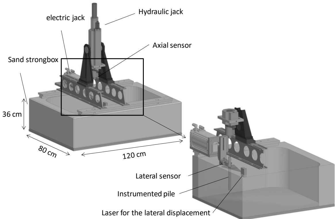
Figure 1. Experimental set up (inside dimensions)
