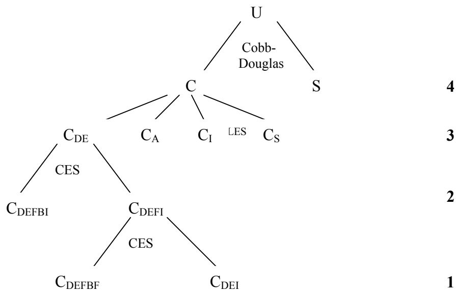
Figure 4 : Households consumption
