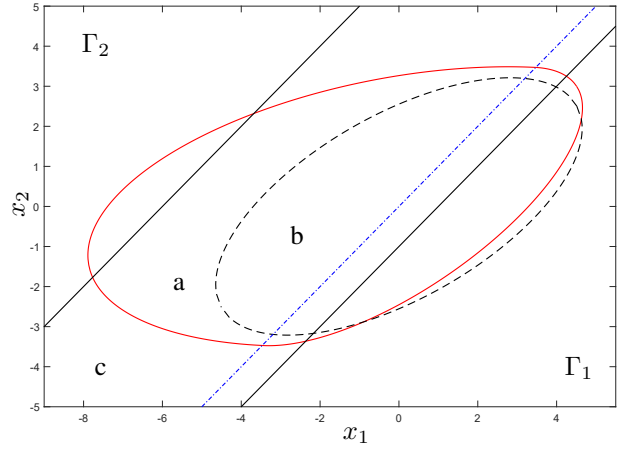
Fig. 1. Example 1 - (a). RAC obtained considering asymmetric bounds; (b). RAC obtained considering a symmetric worst case; (c) Region of linear behavior, i.e. \{x \in \mathbb{R}^2 \mid -1 \leq Kx \leq 6\} . The dash-dotted line divides the space in regions \Gamma_1 and \Gamma_2 .
