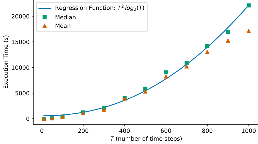
Figure 7: Time-Expanded SSP computation time depending on T , expressed in seconds.
