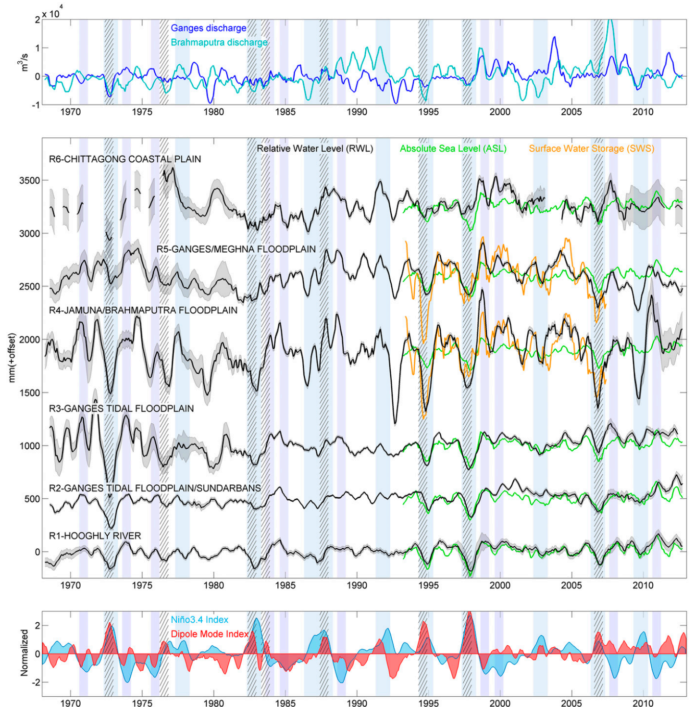
Fig. 2. (Top) Deseasonalized anomalies (subtracting the long-term mean) of Ganges and Brahmaputra discharge time series. (Middle) Regional RWL reconstructed for the 6 regions over 1968 to 2012 (black line). Superimposed are the deseasonalized anomalies of the ASL from altimetry (green line) and the normalized deseasonalized anomalies of the SWS (orange line). (Bottom) Normalized Niño3.4 index (blue shade) and normalized Indian Ocean Dipole Mode index (red). A 6-mo running window was applied to all of the monthly time series. The light blue stripes indicate the El-Niño years and the light purple stripes indicate the La Niña years. The black hatched stripes correspond to the positive IOD years.
