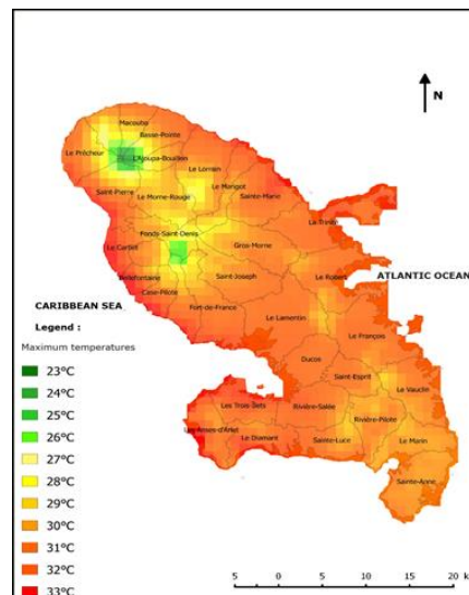
Figure 11: Maximum annual average temperatures (scenario RCP 4.5, 2071-2100). (Source: Météo-France) 14 .
