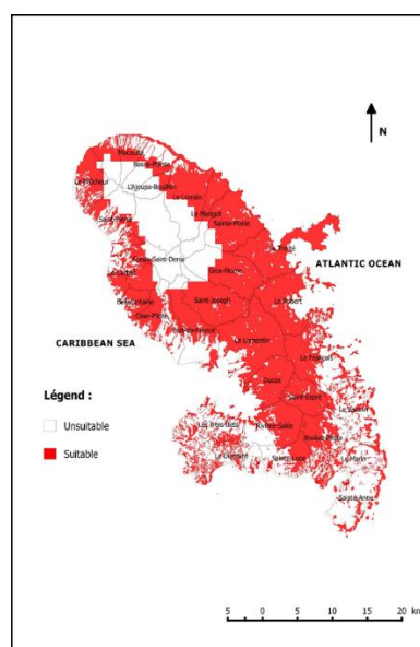
Figure 9: Pedoclimatic zoning of Coffea liberica in Martinique.
