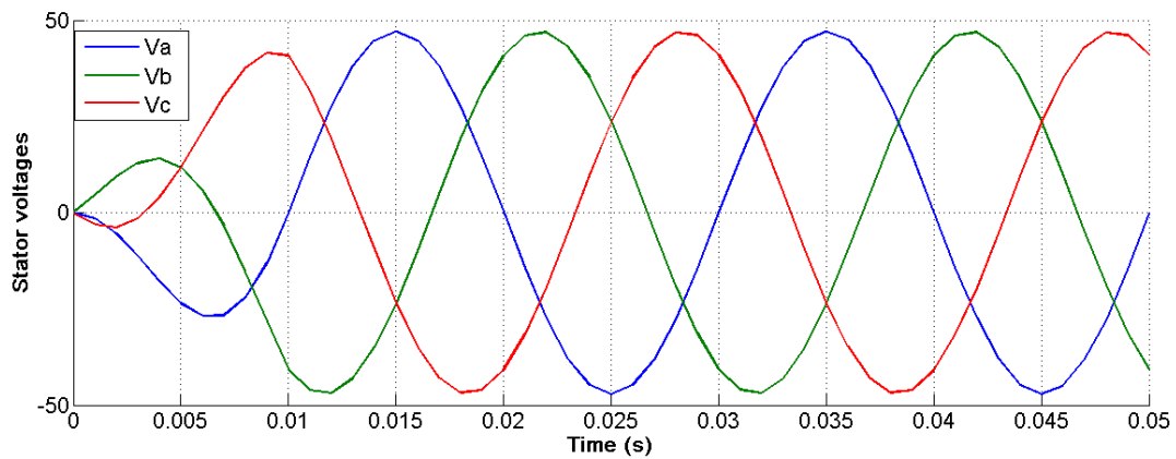
Fig. 7: Stator voltages of the vacuum PMSG
