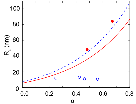
FIG. 6. Elastic and plastic relaxation in axial nanowire heterostructures. The elastic and plastic domains are separated by a line corresponding to the calculated R_c for \text{In}_{0.8}\text{Ga}_{0.2}\text{As}/\text{GaAs} (dashed blue) and \text{InAs}/\text{GaAs} (solid red). Above the line, theory predicts plastic relaxation. The circles indicate the experimental data from dislocation-free (open) and plastically relaxed (solid) structures.
