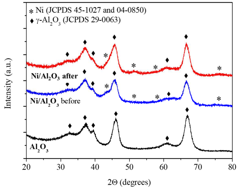
Figure 2. XRD pattern of 10wt% Ni/ \gamma - Al_2O_3 catalyst before and after plasma treatment.
