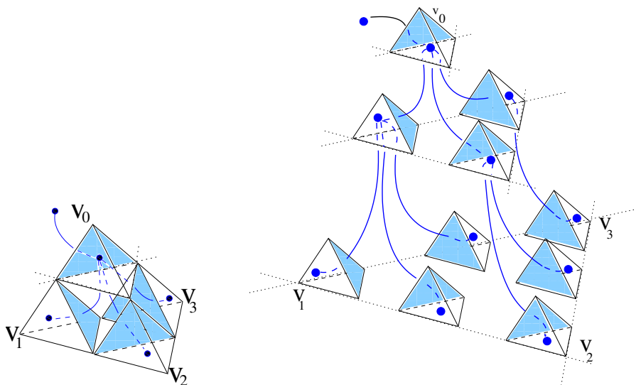
Figure 3: (Taken from [7]) Example of spanning tree in the (dual) graph, namely a selection of acyclic paths made of arcs, visiting all the nodes of the (dual) graph ( r = 1 , left and r = 2 , right).
