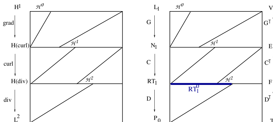
Figure 1: The de Rham complex for the continuous spaces (left) and for Whitney differential forms (right).
