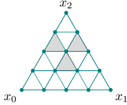
Figure 2: Points of the principal lattice for \mathcal{P}_4^- \Lambda^0(T) , where T is a 2-simplex. The node with barycentric coordinates (\frac{1}{4}, \frac{1}{4}, \frac{2}{4}) in T is shared by the three gray small triangles.
