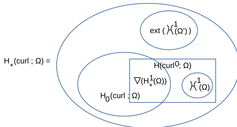
Figure 5: A visualization of the subspaces we consider in H_*(\text{curl}; \Omega) . All the functions in the rectangle are in H(\text{curl}^0; \Omega) = \nabla H^1(\Omega) \oplus \mathcal{H}^1(\Omega) . Here, \nabla H_*^1(\Omega) \subset \nabla H^1(\Omega) , moreover \nabla H_*^1(\Omega) \subset H_0(\text{curl}; \Omega) \cap H(\text{curl}^0; \Omega) since the elements of \nabla H_*^1(\Omega) are gradients, with a constant value on each connected component of \partial\Omega .
