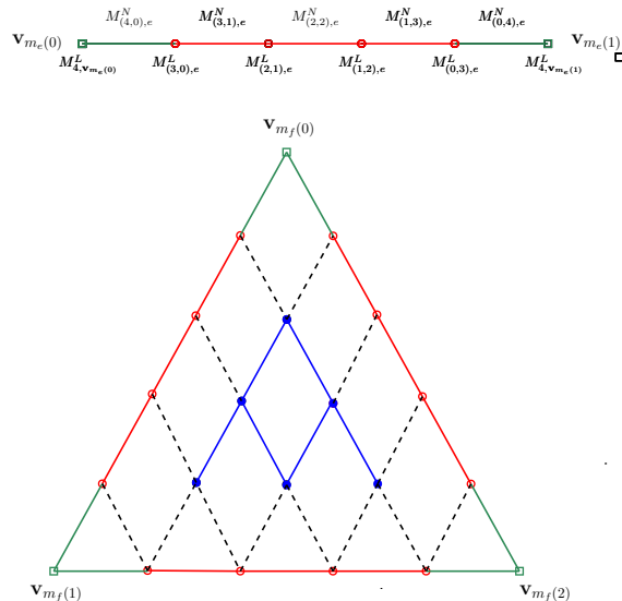
Figure 6: On the top an example of edge subgraph \mathcal{G}_e^* . On the bottom, in blue, an example of face subgraph \mathcal{G}_f ; in red and green the three subgraphs of the edges on the boundary of f , in black, other arcs of the graph that are not on any face or edge subgraph.
