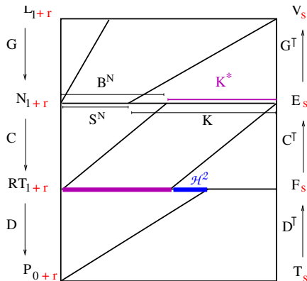
Figure 4: A graphical summary of the structure of the basis of RT_{r+1}^0 and its construction (in the case \beta_2(\Omega) = 0 ). Here, K^* = \mathring{J}_{1,CB} and K = \mathcal{J}_{1,CB} , with or without B depending on \beta_1(\Omega) .
