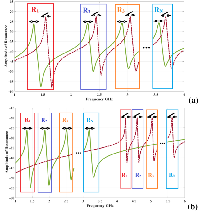
Fig. 5. Data encoding strategies (a) crisscross (b) plain.
