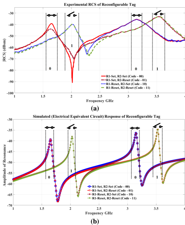
Fig. 7. RF response of electronically rewritable chipless RFID tag on paper substrate (a) Experimental (b) Electrical equivalent model.
