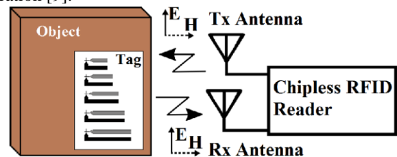
Fig. 1. Bistatic Radar used for RCS measurements of chipless RFID tag.
