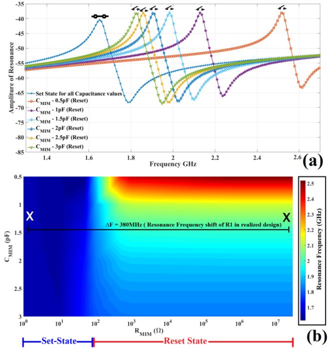
Fig. 4. Dependence of resonance frequency on C_{MIM} and R_{MIM} (a) Resonance Pattern, R_{MIM} in set case is 1\Omega and in reset case is 1\text{M}\Omega (b) Resonance frequency map.
