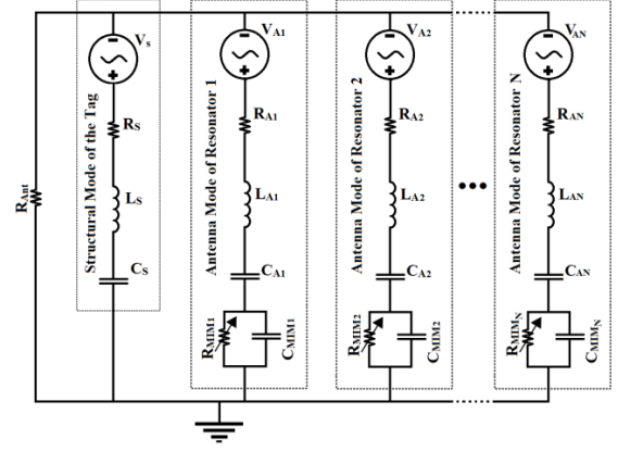
Fig.3. Electrical model of electronically re-writable chipless RFID tag.
