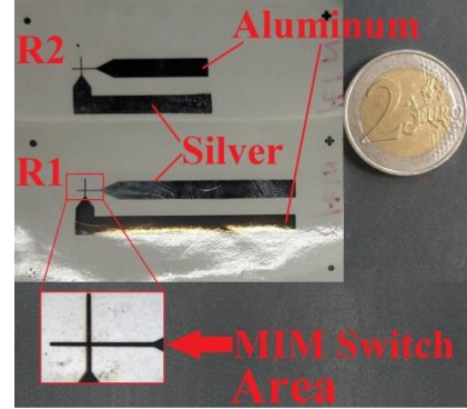
Fig. 6. Photograph of fabricated electronically rewritable chipless RFID tag with microphotograph of MIM switch area in the inset.
