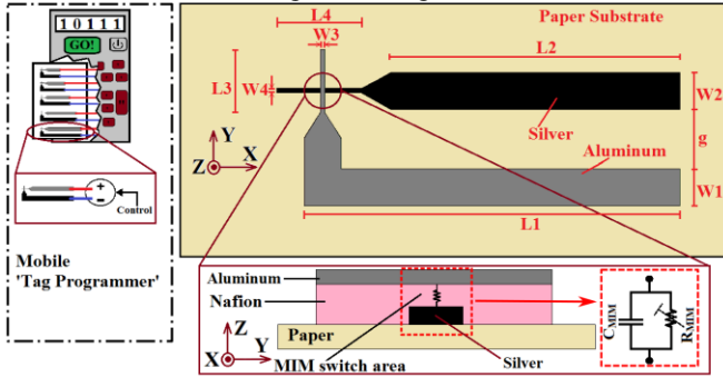
Fig. 2. Topology of REP used and electrical model of MIM Switch (Layers not up to scale). Inset shows a cut out view of a mobile ‘Tag-Programmer’. W1=W2=g=3\text{mm} , W3=160\mu\text{m} , W4=140\mu\text{m} . L3=3\text{mm} , L4=4\text{mm} . Resonator1 (R1): L1=37\text{mm} , L2=30\text{mm} , Resonator2 (R2): L1=18\text{mm} , L2=11\text{mm} .
