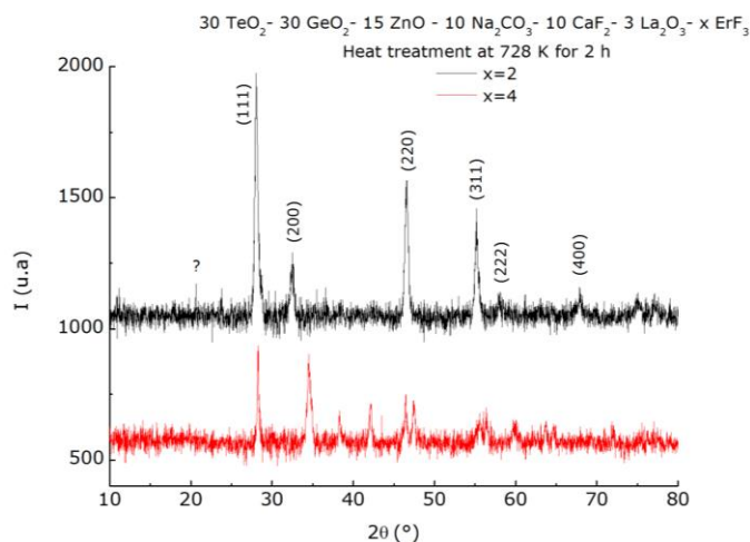
Figure 2. X-ray diffraction patterns of two heat-treated glasses. The indexation mentioned in the black diffractogram corresponds to the Miller indices of the CaF 2 cubic phase Fm-3m.
