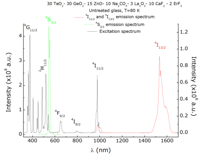
Figure 4. “2 ErF 3 ”-doped and thermally untreated glass excitation and emission spectra recorded at 80 K.
