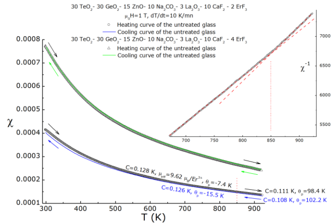
Figure 7. MKSA magnetic susceptibility of “2 ErF_3 ”- and “4 ErF_3 ”-doped glasses, measured upon cycling around the crystallization temperature, and zoom of the high temperature inverse magnetic susceptibility of the former glass. Between the black and the blue curves, a 15 mn-long stage at 930 K is applied.
