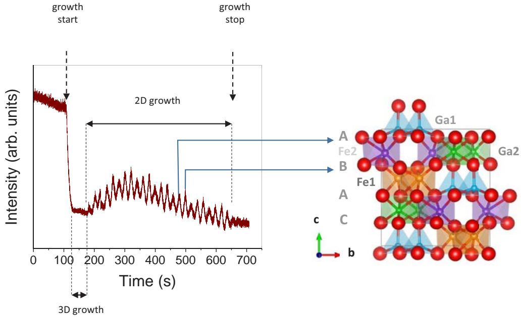
FIG. 2. Fluctuation of the intensity of a spot in the zero-order Laue zone during RHEED monitoring of the 7-nm GFO film growth. Each oscillation corresponds to the deposition of one fourth of a GFO cell, that is, to a layer of transition-metal/oxygen polyhedra.
