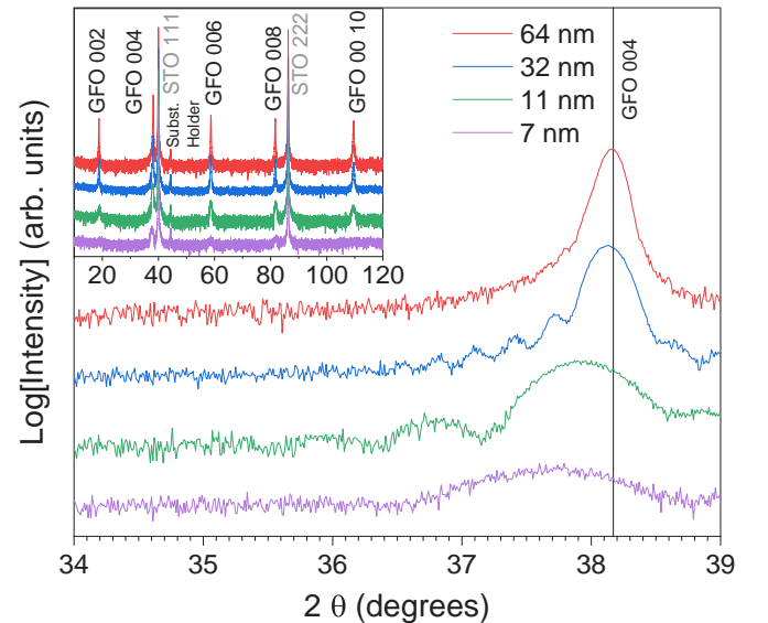
FIG. 3. X-ray diffractograms of the deposited GFO thin films in the \theta - 2\theta mode, with a focus on the GFO 004 peak, the vertical line at 2\theta = 38.17^\circ indicates the angle observed for bulk GFO x = 1.4 ( c = 0.9422 nm) [17].
