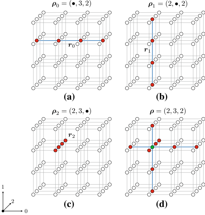
Fig. 1 Illustration of tensor fibers and crosses definition, for a given multi-index \rho . The residual restriction onto its corresponding fibers, r_* , are also indicated
