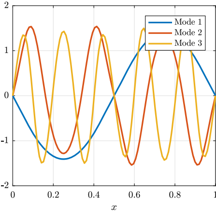
(b) First 3 x-dir. modes: \{\mathbf{w}_0^m\}_{m=1}^3
