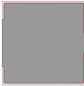
Figure 5: Density \rho = 0.5 of the initialization structure for the cantilever test case (the boundary of \Omega is the red line)
