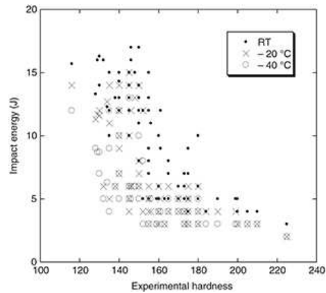
Figure 2. Experimental values of impact energy at the three investigated temperatures plotted versus experimental hardness at RT.
