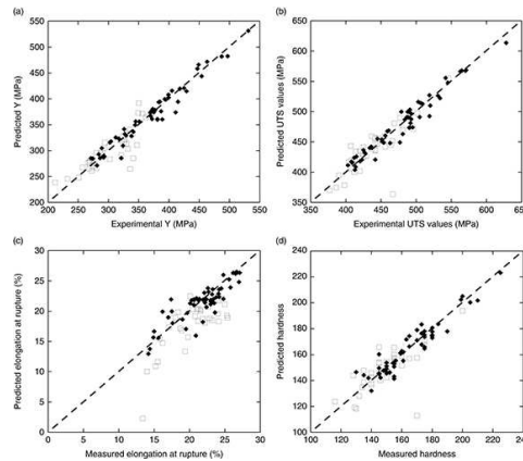
Figure 1. (a) Correlation between predicted and experimental values of Y, (b) UTS, (c) A and (d) HB. Solid symbols refer to fully ferritic alloys, open symbols to those containing more than 2% pearlite.
