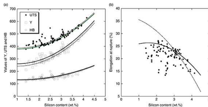
Figure 3. Effect of silicon content on the RT mechanical properties of studied cast irons: (a) Y, UTS and HB; and (b) A. Symbols are the experimental data, dotted lines are calculated for an average carbon content of 3.5 wt.% and a nodule count of 300 mm^{-2} ; solid lines are calculated accounting for other relevant elements (Cu: 0.1, Ni: 0.1 and S: 0.01, wt.%).
