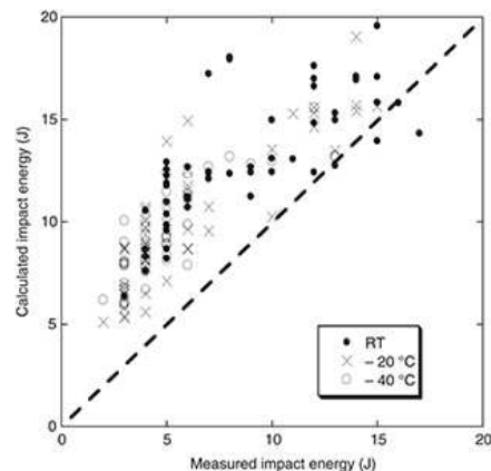
Figure 4. Comparison of experimental and calculated impact energies for fully ferritic alloys.
