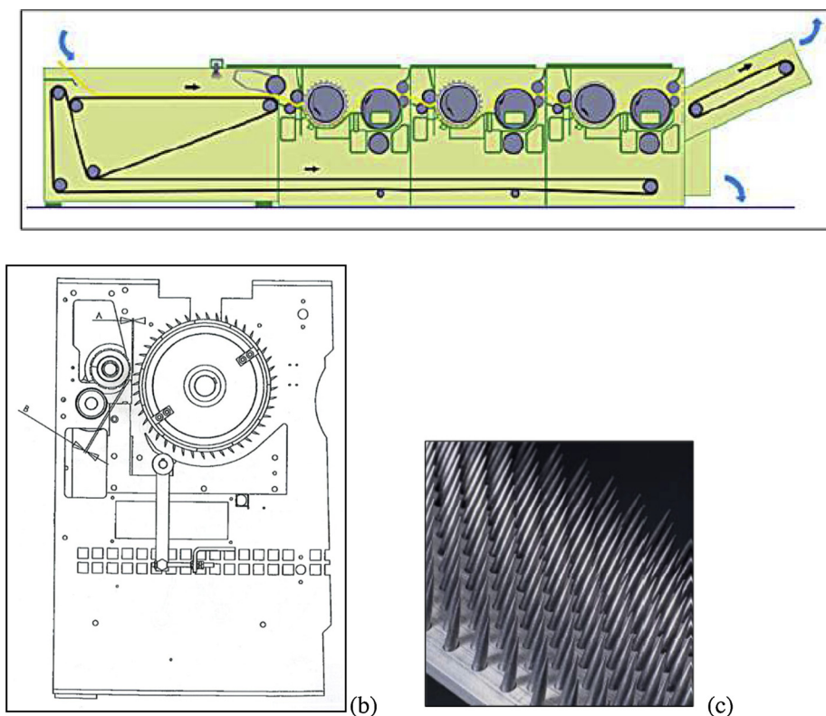
Fig. 4. Laroche (France) Cadette 1000 “all fibre” extraction device used in this study (from Laroche company website). (a) Material path along the opener (in yellow on the drawing), from the feed belt (left) to the exit belt (right). (b) Detailed view (from left to right) of the pair of rolls needed for feeding (smooth roll down and grooved roll up), and the fibre extraction roller (cylinder equipped with nails), all three located at the module inlet. (c) Photograph of the nails of the extracting roller in module 1.
