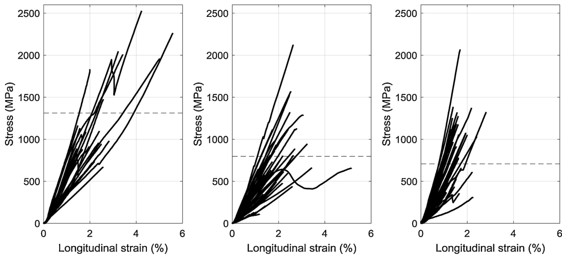
Fig. 8. Tensile stress-strain curves of nettle fibres from the batches Y2-S2-FS manually extracted (a), Y2-S1-TS with manual extraction (b) and Y2-S1-TS with mechanical extraction (c).
