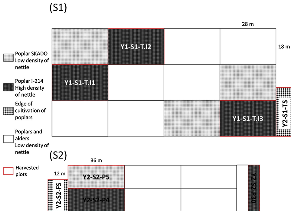
Fig. 2. Experimental designs at the two phytomanaged field sites, Tavaux (S1) and Fresnes-sur-Escaut (S2). The sampled plots are in dark grey (I214 plots) and light grey (Skado), on which nettles were collected. Full description of the sites is provided in (Phanthavongsa et al., 2017). Nettles were also collected in the edge of the poplar plots.
