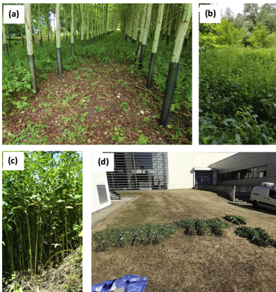
Fig. 3. Photograph the plots and the crops. (a) Plot No. Y1-S1-T.I3 after harvest, (b, c) Nettles in the plot No. Y1-S2-TS, at the wood-edge, and (d) Crop of Y2-S2-(FS, P4, P5, P30).
