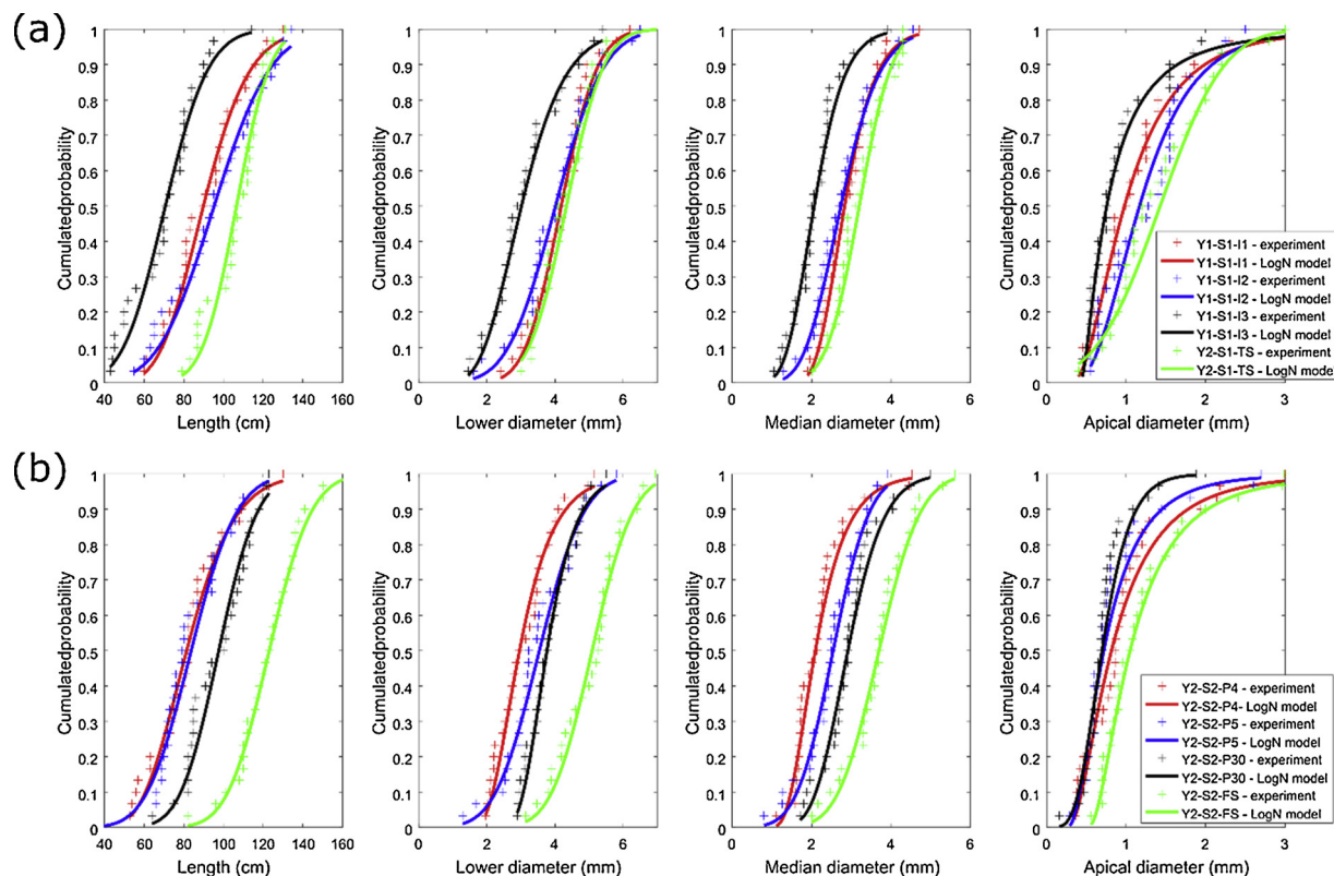
Fig. 5. Statistical distribution of the nettle stem features (length and diameter) as a function of the location in the plant and of the harvesting site: S1 (a) and S2 (b).
