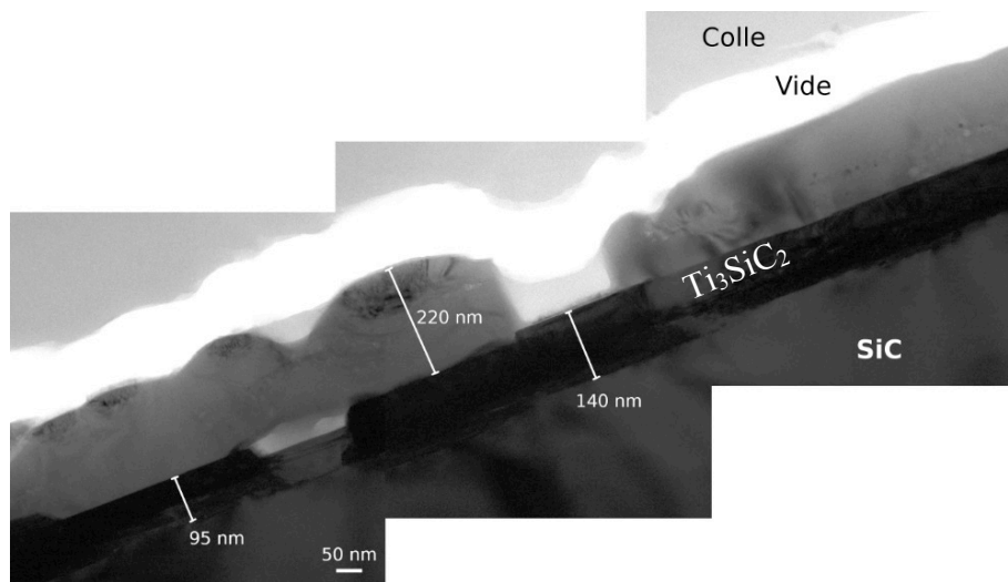
Figure 2. Cross-sectional TEM image of the same sample as in figure 1. Ti_3SiC_2 covers completely the surface of the SiC substrate and is itself covered by a Al oxide layer.
